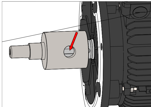
Fig. 3.4.2 Align keyseat with shaft hole.
