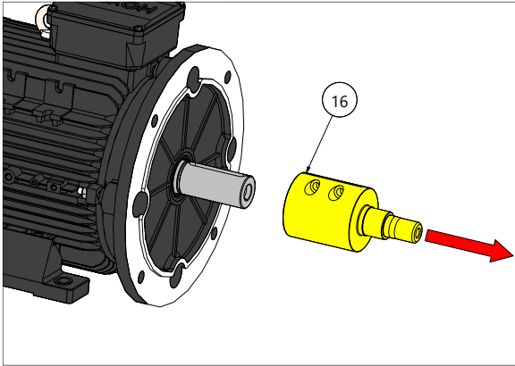
Fig 3.3.17 Remove the shaft [16].
