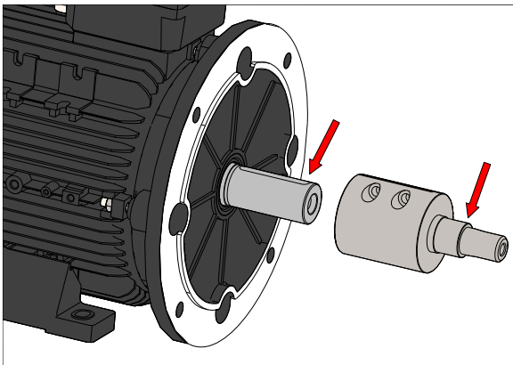
Fig. 3.4.1 Degrease the motor shaft and pump shaft before assembly.
