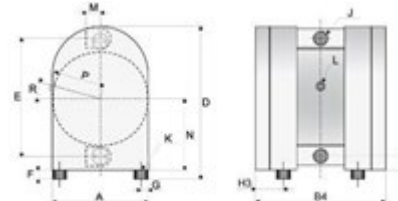
Standardpumpe PTFE
