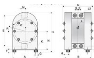
Twinpumpen TT
