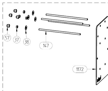
Pressure booster – TF (left side)
