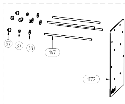
Pressure booster – TF (right side)
