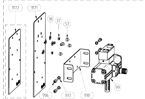
Pressure booster – TF (right side)
