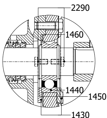
DETAIL B: 58-80 / 86-100
