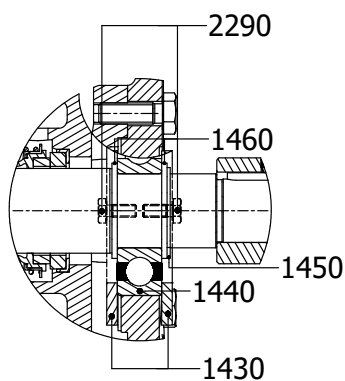
DETAIL B: 15-50 / 23-65
