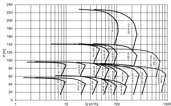
3600 rpm/60 Hz
