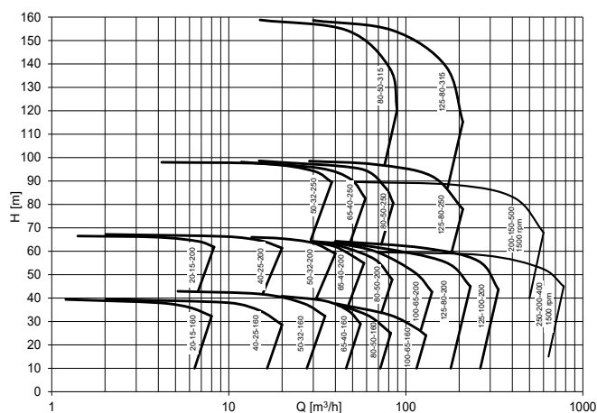
3000 rpm/50 Hz
