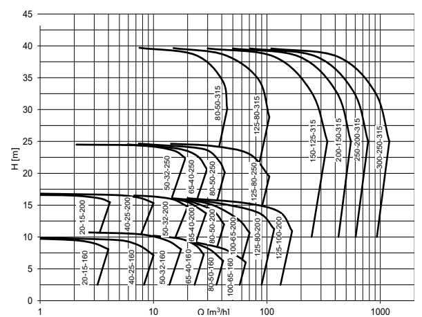
1500 rpm/50 Hz
