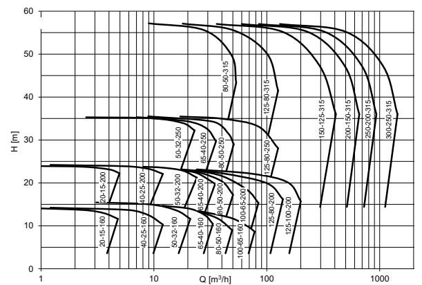
1800 rpm/60 Hz
